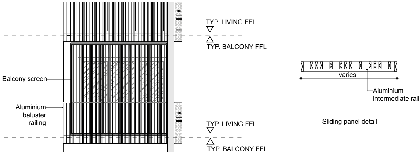
Front Elevation
